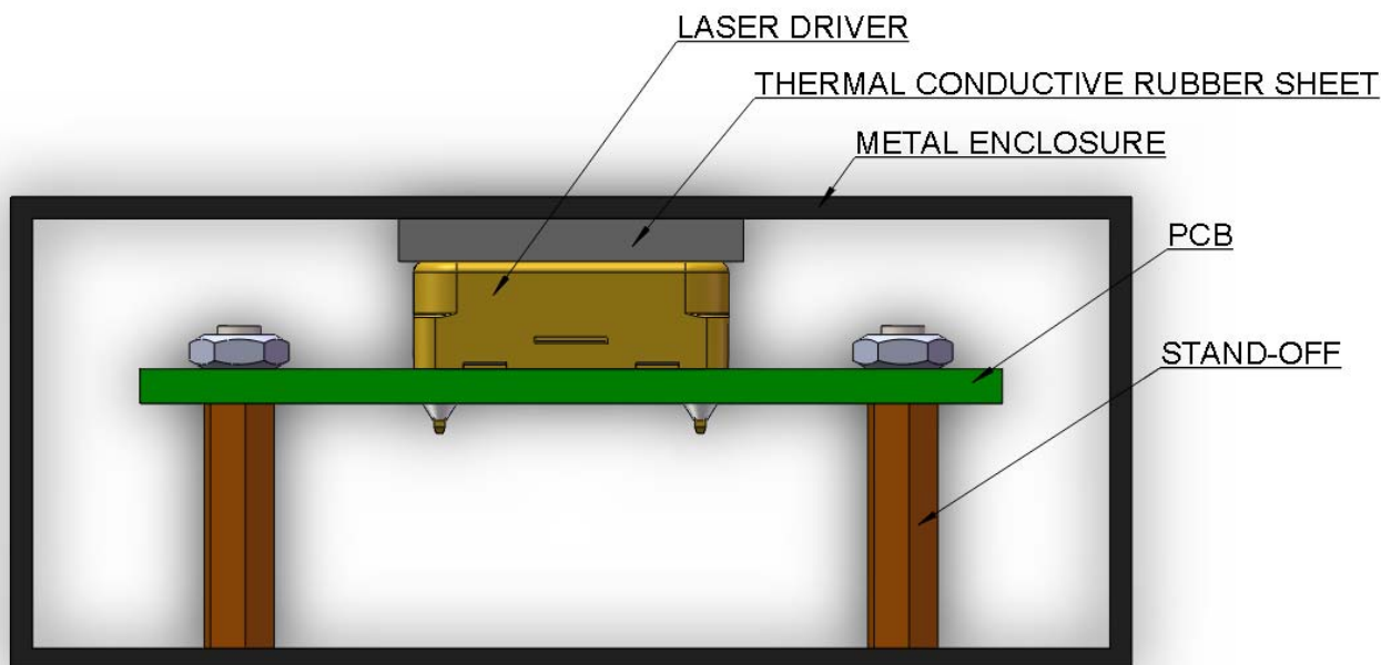
Figure 9.1 Transferring Heat with Metal Enclosure
