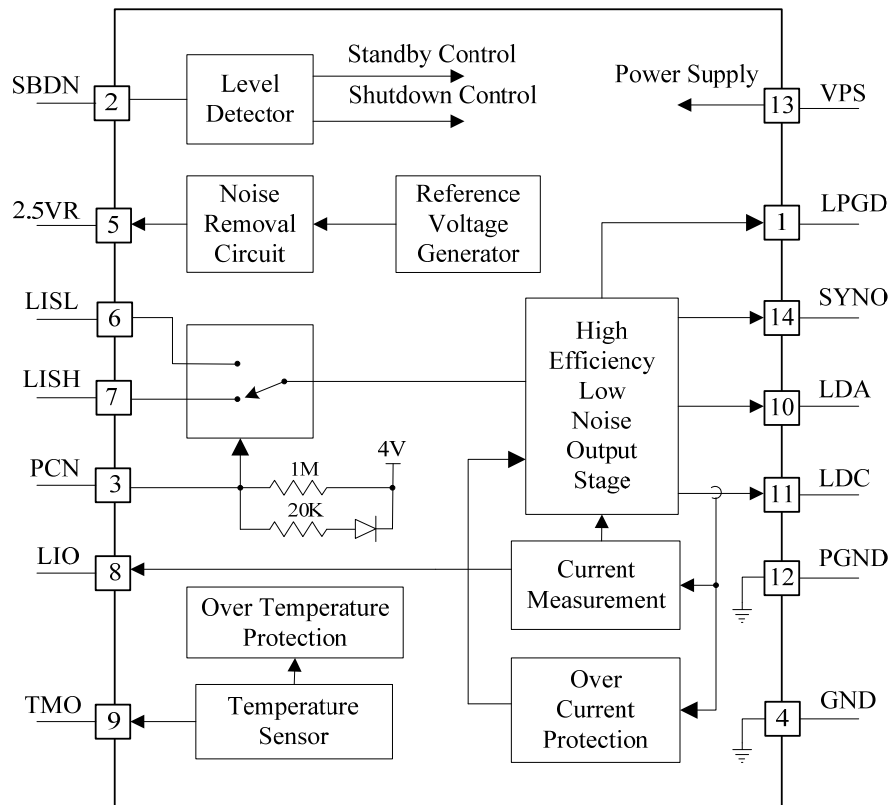
Figure 3. Internal Block Diagram of ATLS500MA212
