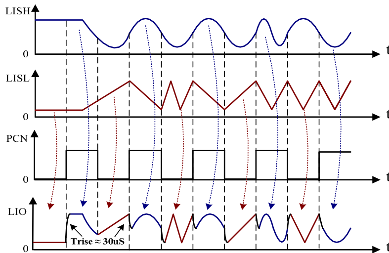
Figure 6. Digitally Controlled Analog Modulation Principle
