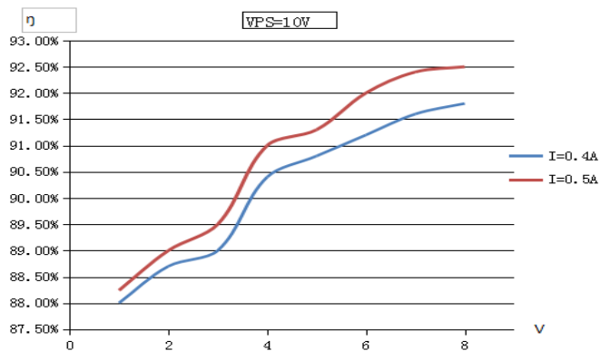
Figure 11. The efficiency of the laser driver.
