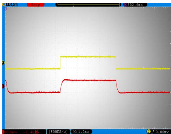
Figure 12. Small Signal Modulation
