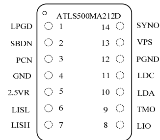
Figure 2. Pin Names and Locations
