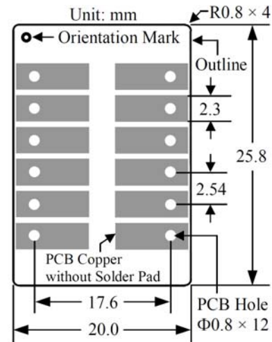
Figure 7. Top View of the PCB Foot-print
