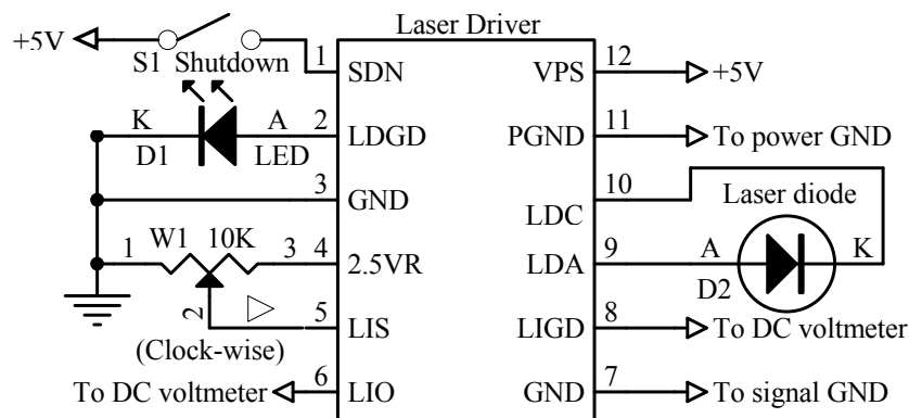
Figure 4.2. A Typical Stand-alone Application Schematic for ATLS500MA201D-PD
