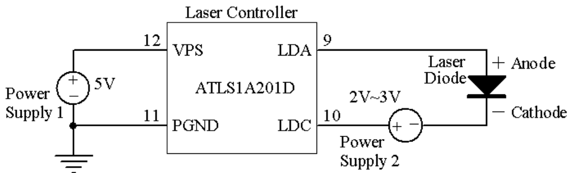
Figure 7. Driving High Voltage Laser Diodes
