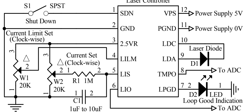
Figure 4.1 Typical Stand-alone CW Operation Schematic for ATLS500MA103
