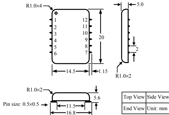
Figure 19. Dimensions of the SMT Package Controller
