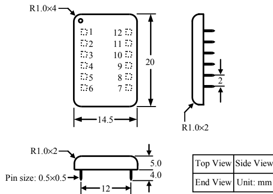
Figure 12. Dimensions of the DIP Package Controller
