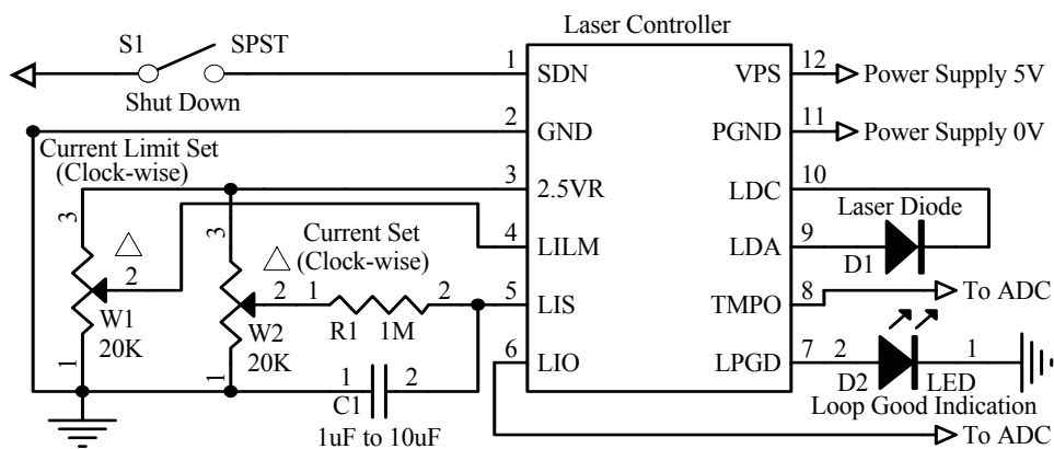
Figure 4.2. Typical Stand-alone CW Operation Schematic for ATLS500MA103-PD
