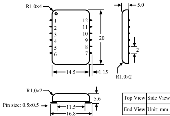
Figure 13. Dimensions of the SMT Package Controller
