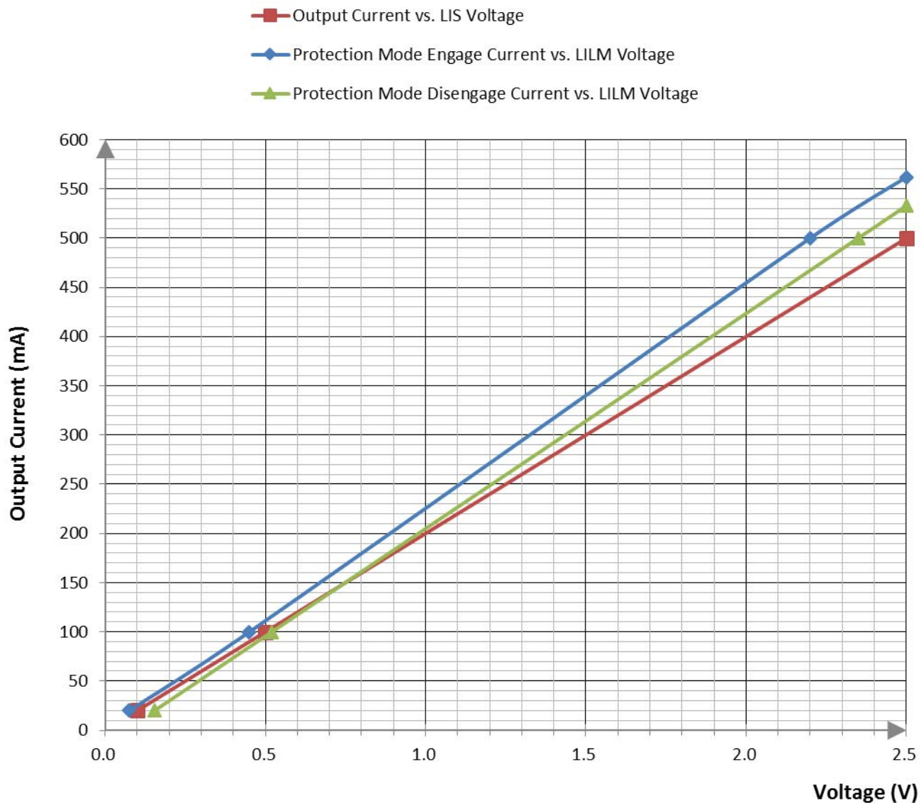
Figure 11. Output Current vs. LIS and LILM Voltage
