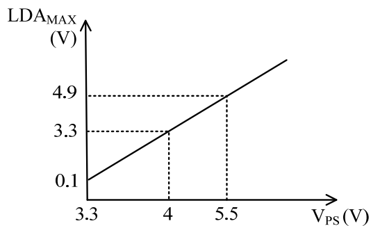
Figure 6. Relationship between VPS and LDA MAX
