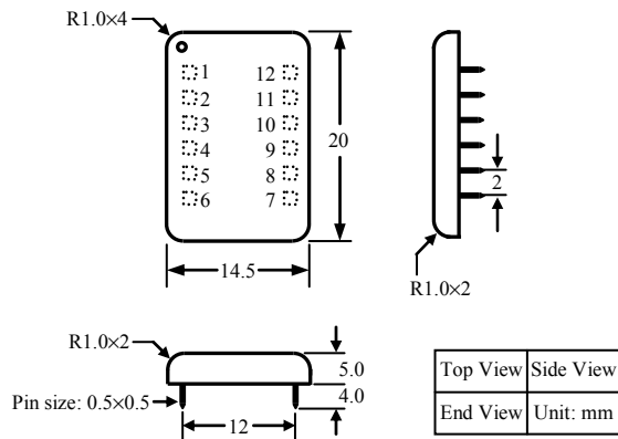
Figure 12. Dimensions of the DIP Package Controller
