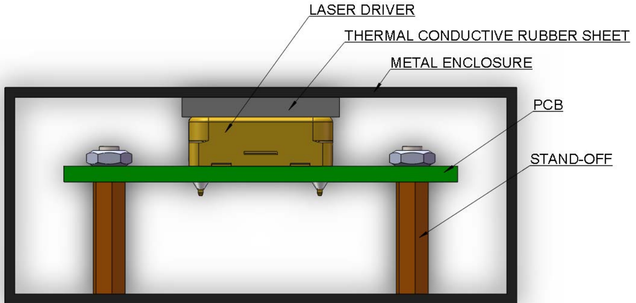
Figure 8.1 Transferring Heat with Metal Enclosure
