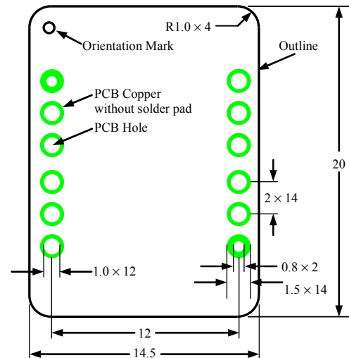
Figure 14. Top Side PCB Foot-print for the DIP Package
