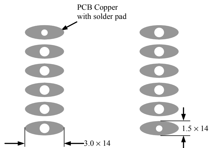
Figure 14. Top Side PCB Foot-print for the DIP Package
