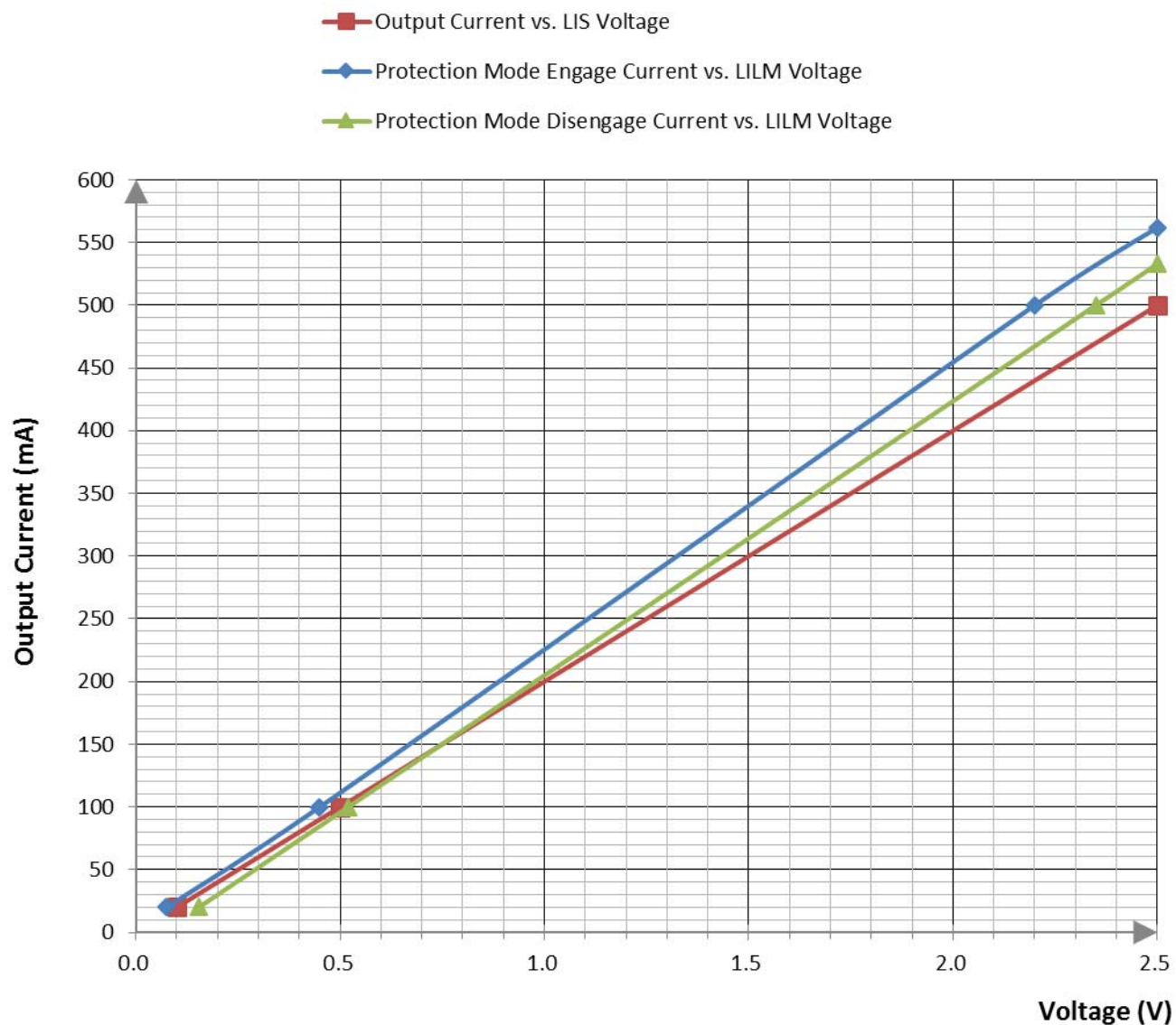
Figure 16. Output Current vs. LIS and LILM Voltage
