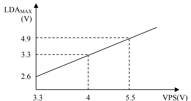
Figure 6. Relationship between VPS and LDA MAX
