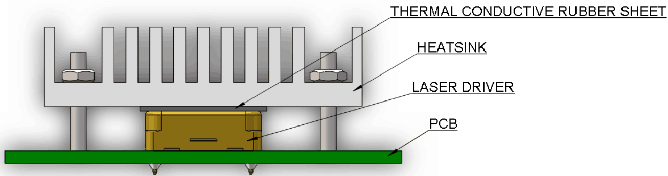
Figure 8.2 Transferring Heat with Heat Sink
