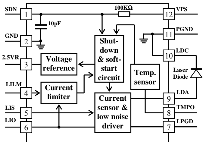
Figure 3. Block Diagram
