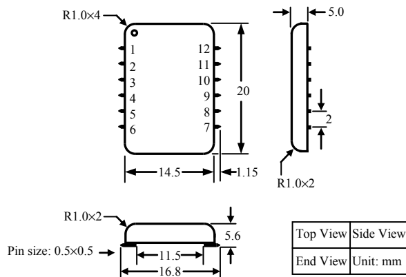
Figure 13. Dimensions of the SMT Package Controller
