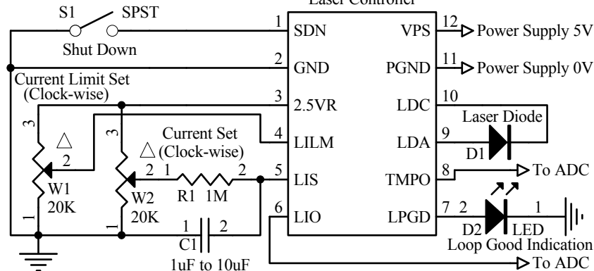
Figure 4.1 Typical Stand-alone CW Operation Schematic for ATLS500MA103
