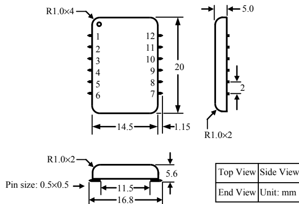
Figure 18. Dimensions of the SMT Package Controller
