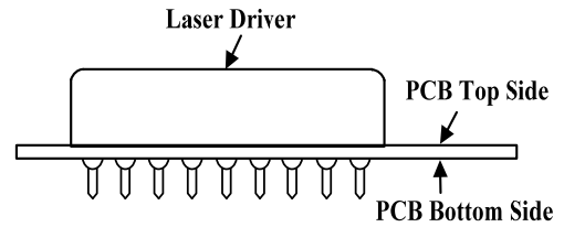
Figure 13. End View of the PCB Foot-print
