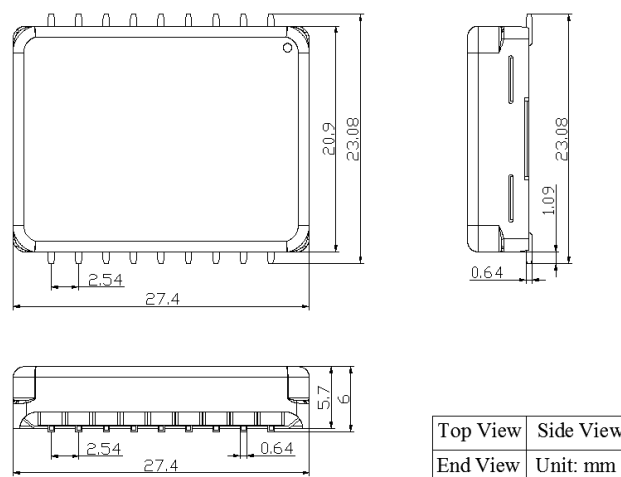
Figure 13. Dimensions of the SMT Package Driver
