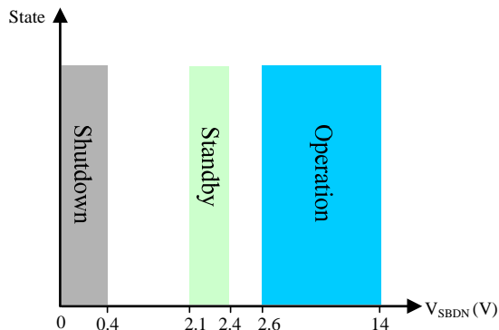
Figure 4. Input Control
