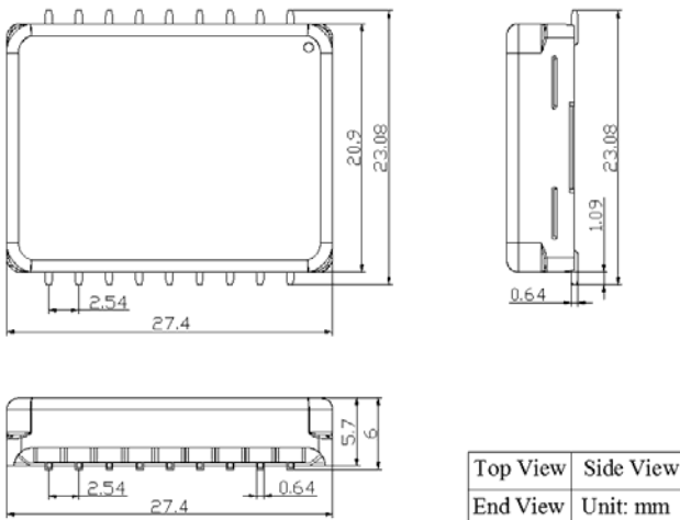
Figure 12. Dimensions of the SMT Package Driver
