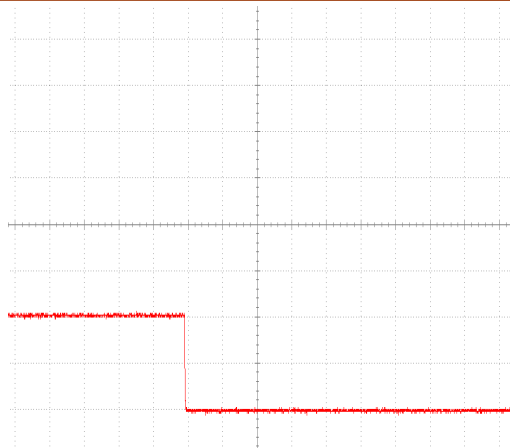
The soft stop of shutdown by both power supply and the switch. When the current is 4A, the voltage is 2V.
