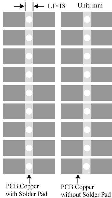
Figure 15. Top View of the Bottom Side PCB Foot-print
