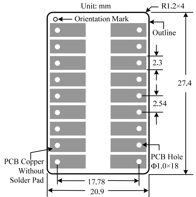
Figure 14. Top View of the Top Side PCB Foot-print
