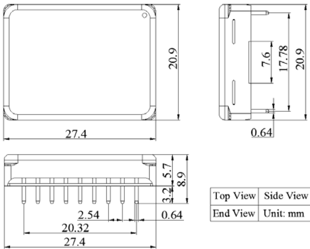
Figure 11. Dimensions of the DIP Package Driver
