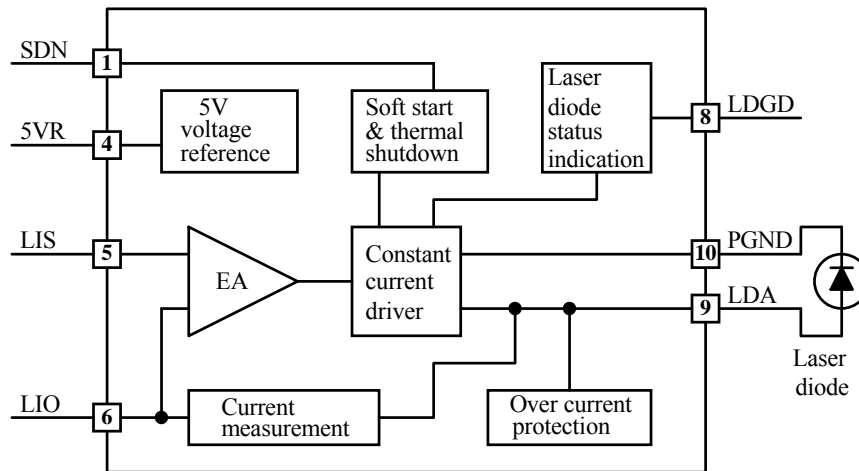
Figure 3. Block Diagram
