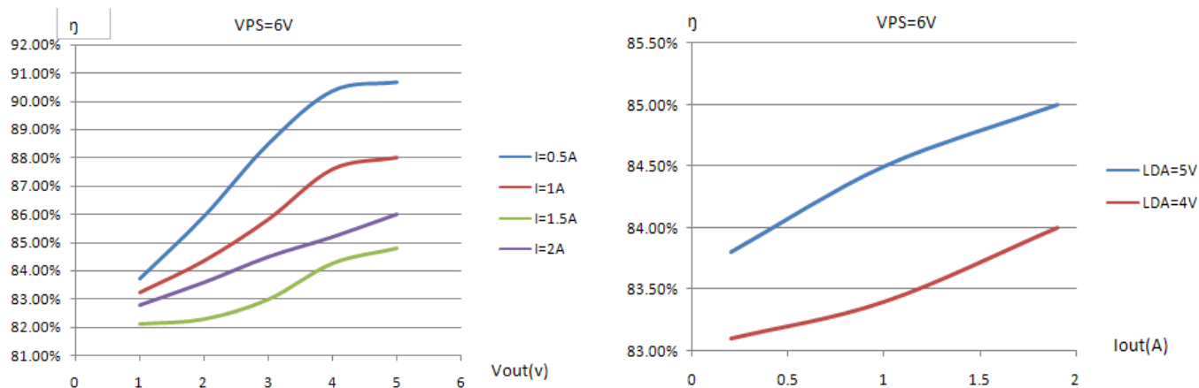
Figure 11. Efficiency of Laser Driver
