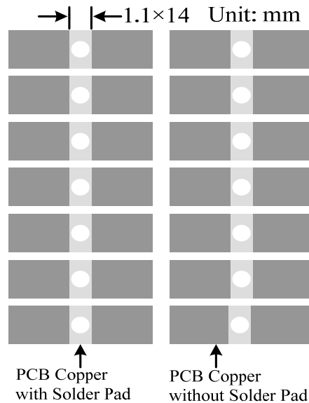
Figure 16. Top View of the Top Side PCB Foot-print Figure 17. Top View of the Bottom Side PCB Foot-print
