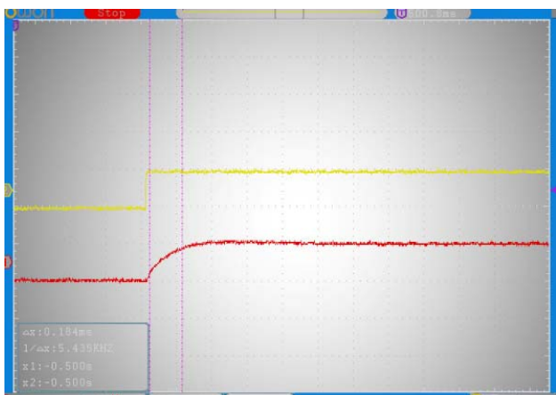
Figure 12.1. The Rise Signal Modulation
