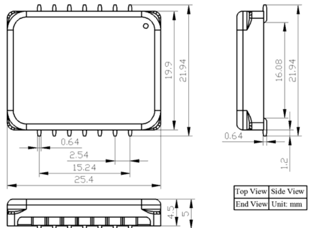
Figure 14. Dimensions of the SMT Package Driver
