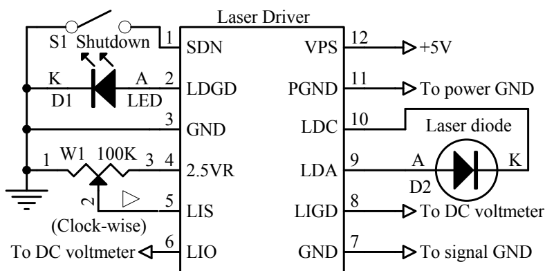
Figure 4.1. A Typical Stand-alone Application Schematic for ATLS2A201D
