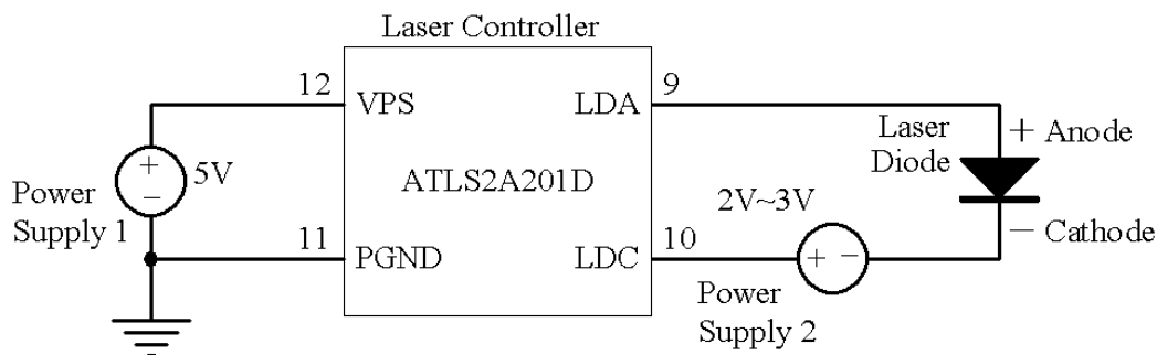
Figure 8. Driving High Voltage Laser Diodes
