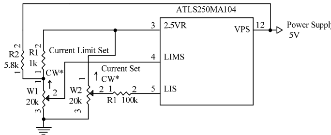
Figure 7. V_{LIMS} setting larger than V_{LIS}
