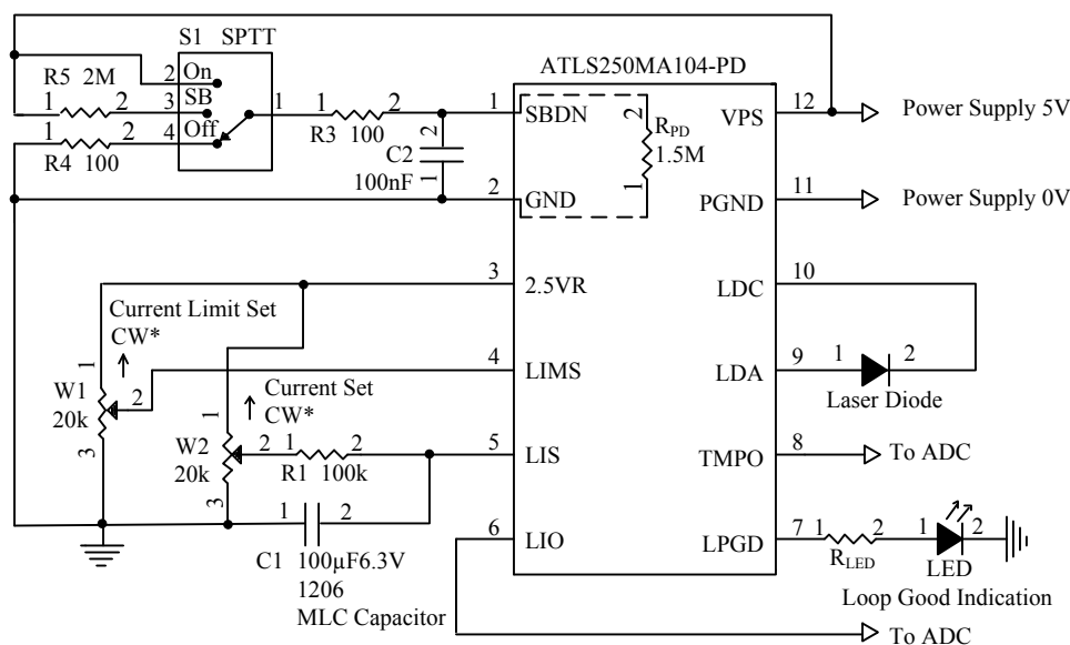
Figure 5.2. Typical Stand-alone CW Operation Schematic for ATLS250MA104-PD
