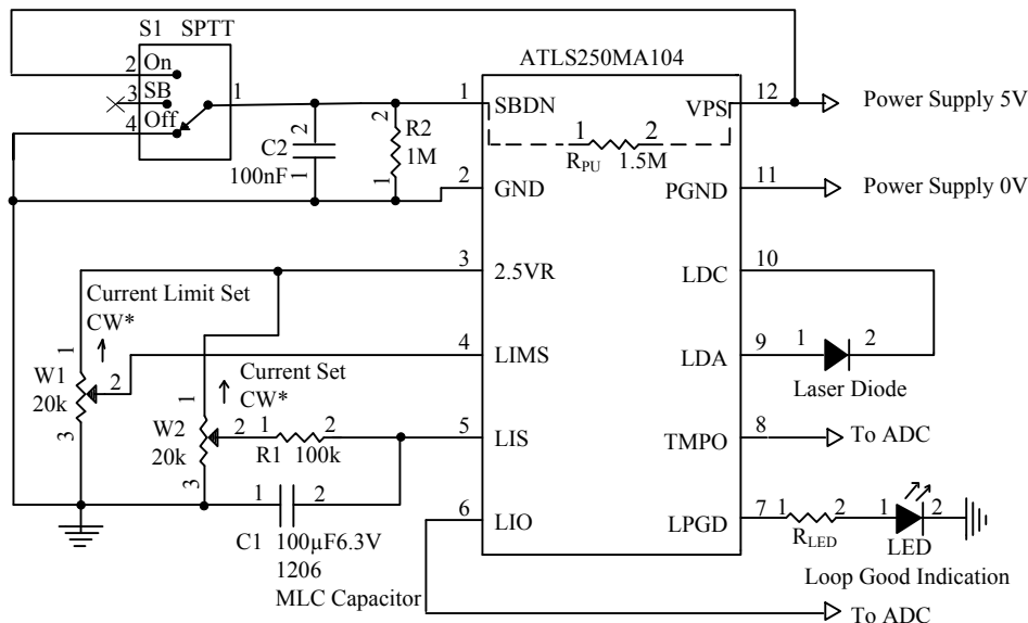
Figure 5.1. Typical Stand-alone CW Operation Schematic for ATLS250MA104
