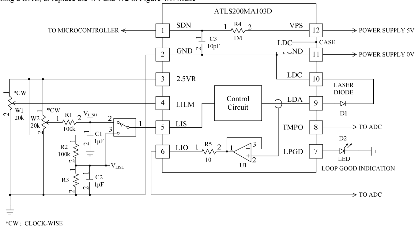
Figure 5. Low Noise Digital Modulation Circuit
