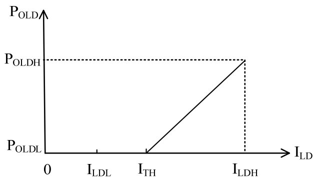
Figure 9. Laser Diode Current I_{LD} vs. Laser Diode Optical Power P_{OLD}
