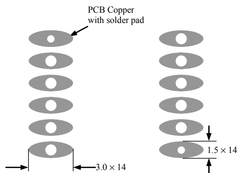
Figure 20. Top View of the Bottom Side PCB Foot-print
