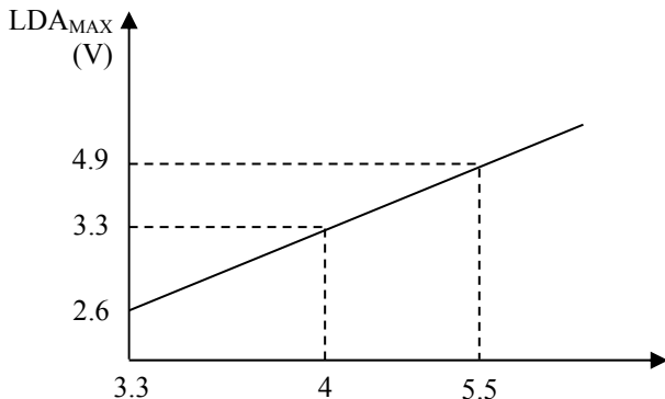
Figure 6. Relationship between VPS and LDA MAX
