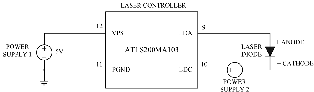
Figure 14. Driving High Voltage Laser Diodes
