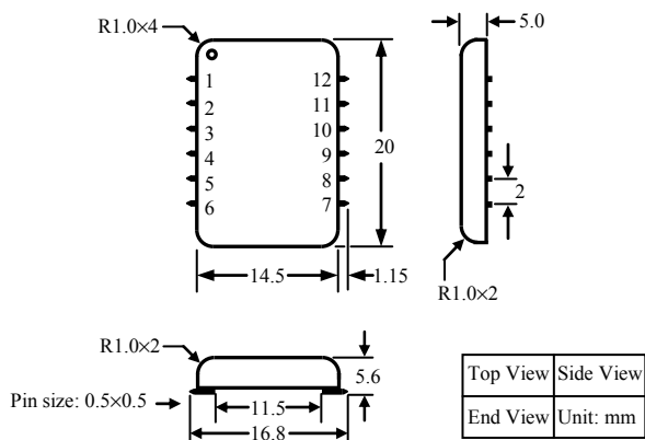
Figure 17. Dimensions of the DIP Package Controller
