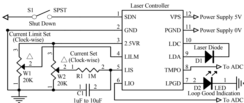
Figure 4.2. Typical Stand-alone CW Operation Schematic for ATLS200MA103-PD
