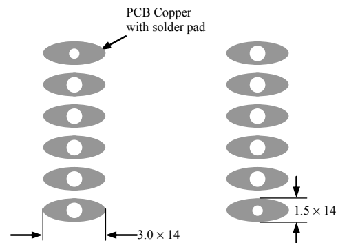
Figure 19. Top View of the Bottom Side PCB Foot-print
