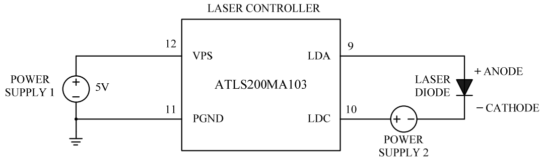
Figure 9. Driving High Voltage Laser Diodes
