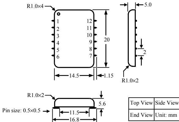
Figure 16. Dimensions of the DIP Package Controller
