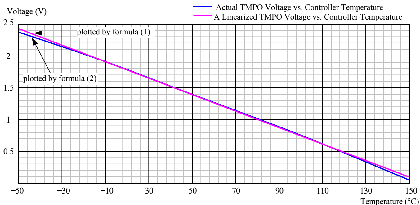
Figure 10. Controller Internal Temperature vs. TMPO Voltage
