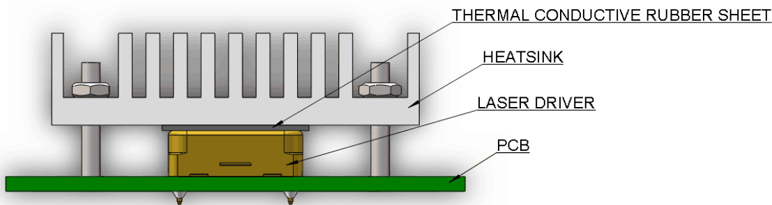
Figure 13.2 Transferring Heat with Heat Sink
