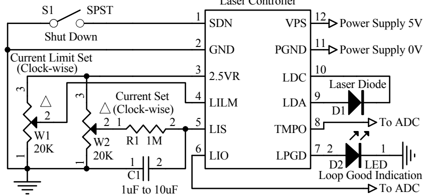
Figure 4.1. Typical Stand-alone CW Operation Schematic for ATLS200MA103
