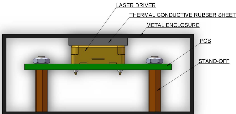
Figure 13.1 Transferring Heat with Metal Enclosure
