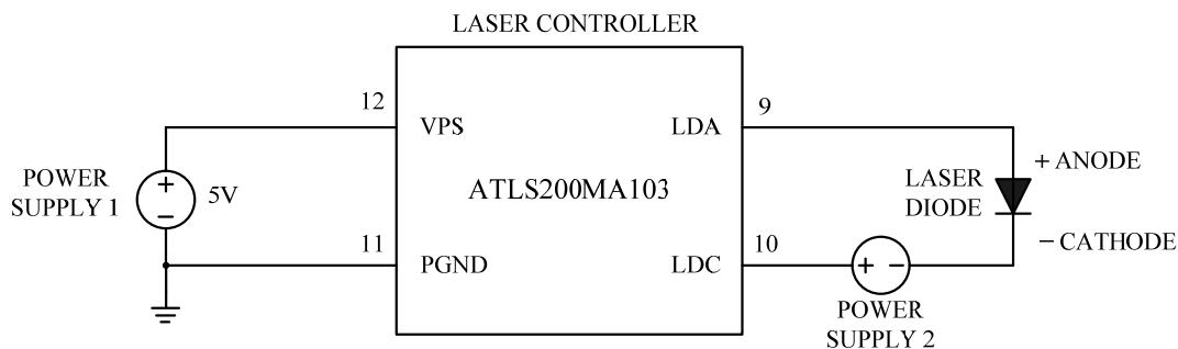
Figure 9. Driving High Voltage Laser Diodes
