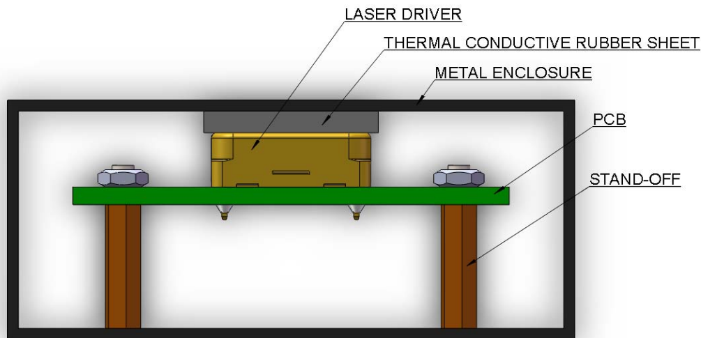
Figure 8.1 Transferring Heat with Metal Enclosure
