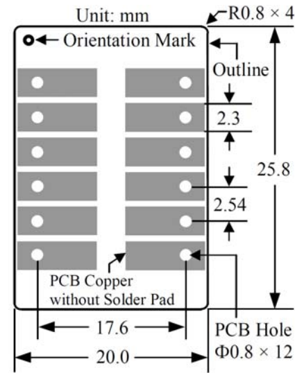
Figure 7. Top View of the PCB Foot-print
