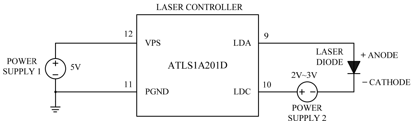
Figure 7. Driving High Voltage Laser Diodes
