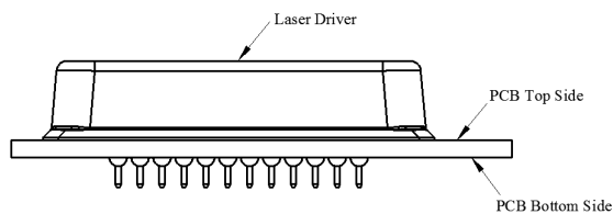
Figure 12. End View of the PCB Foot-print
