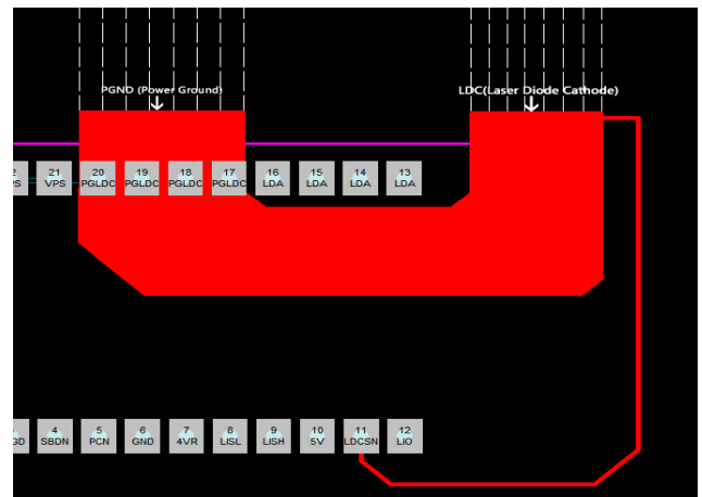
Figure 17. The Layout for the Single-Layer PCB
