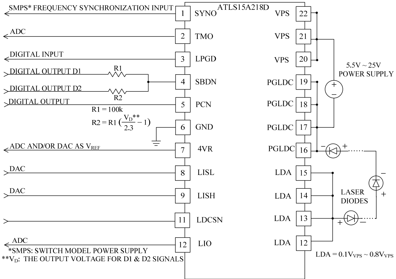
Figure 8. Micro-Controller Based Application Schematic
