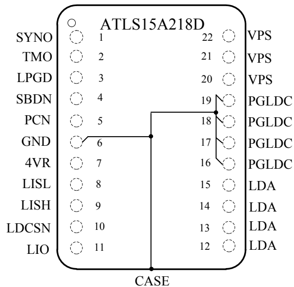
Figure 2. Pin Names and Locations
