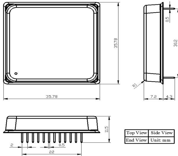
Figure 11. Dimensions of the DIP Package Driver
