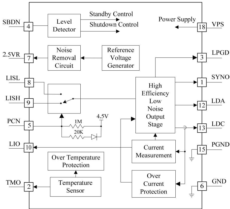
Figure 3. Internal Block Diagram of ATLS15A218
