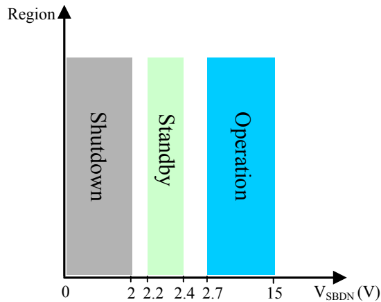
Figure 4. Input Control
