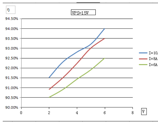
Figure 6. Efficiency of Laser Driver
