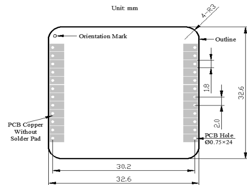
Figure 13. Top View of the Top Side PCB Foot-print
