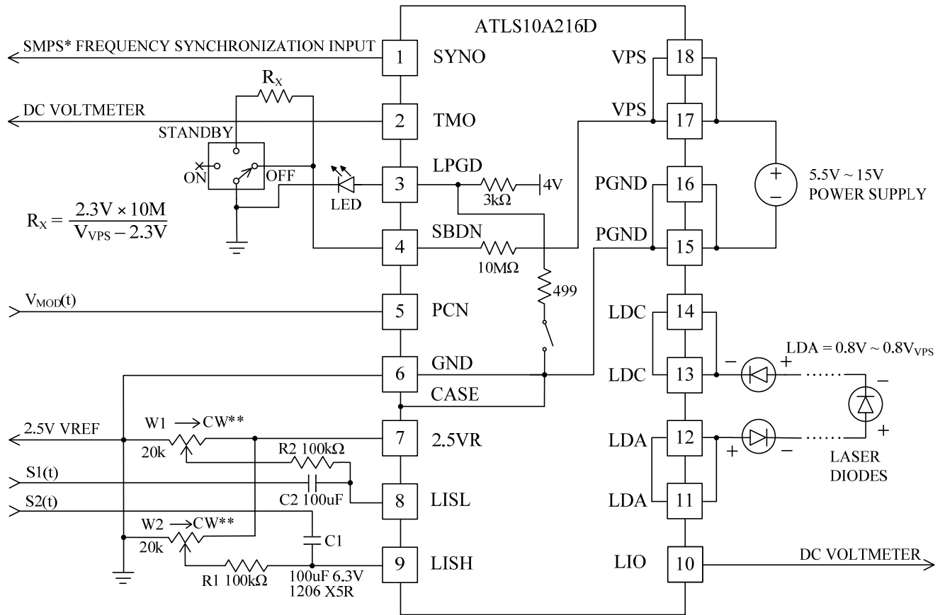
Figure 6. Stand-Alone Application Schematic
