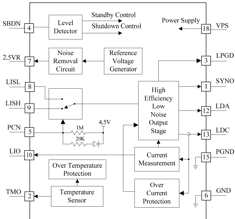
Figure 3. Internal Block Diagram of ATLS10A216
