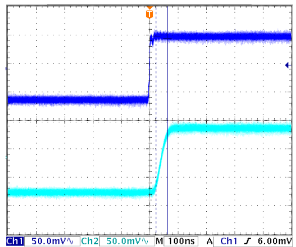
Figure 12.1. Small Signal Rise Time 40ns
