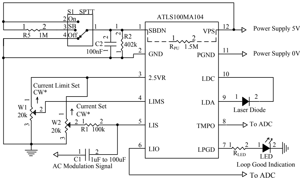
Figure 5.3. Typical AC Modulation with DC bias Schematic for ATLS100MA104
