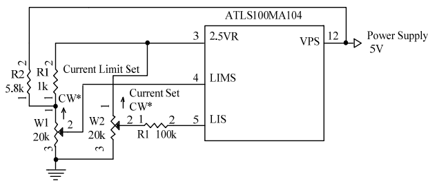
Figure 7. V_{LIMS} setting larger than V_{LIS}
