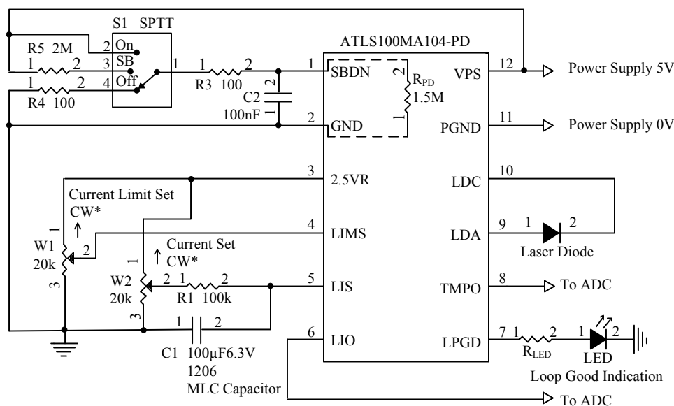
Figure 5.2. Typical Stand-alone CW Operation Schematic for ATLS100MA104-PD
