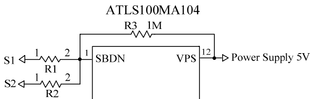
Figure 6. SBDN controlled by microcontroller
