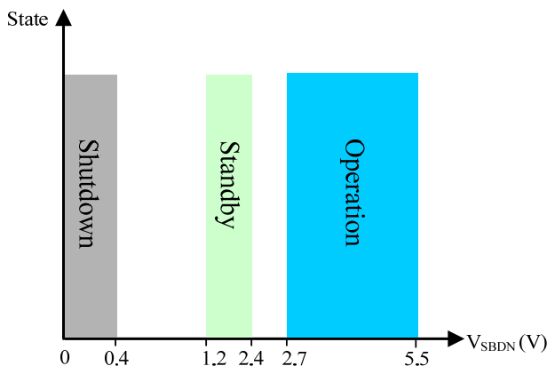
Figure 3. Input Control
