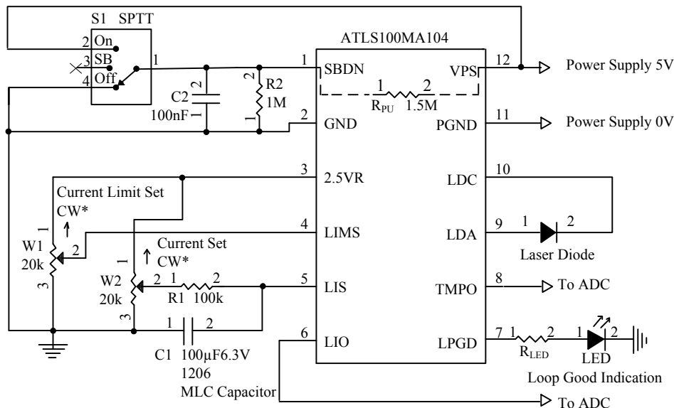
Figure 5.1. Typical Stand-alone CW Operation Schematic for ATLS100MA104
