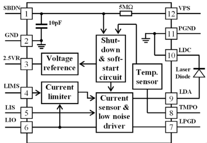
Figure 4. Block Diagram
