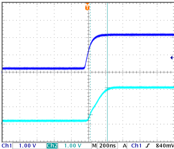
Figure 11.1. Large Signal Rise Time 200ns
