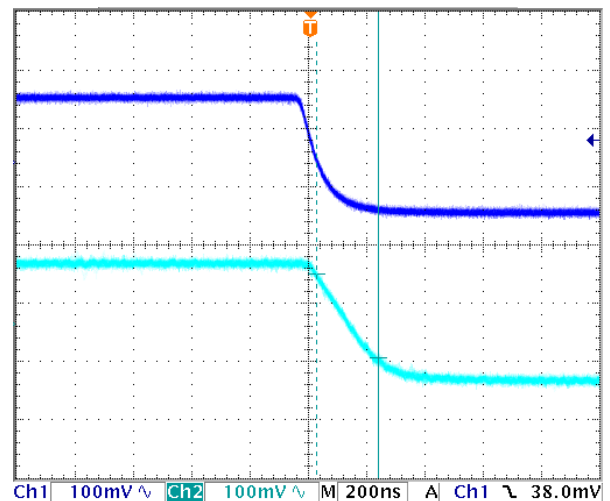
Figure 12.2. Small Signal Fall Time 212ns
