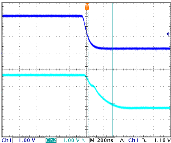
Figure 11.2. Large Signal Fall Time 280ns
