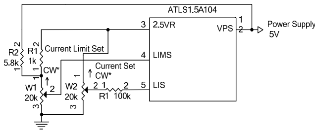
Figure 7. V_{LIMS} setting lager than V_{LIS}
