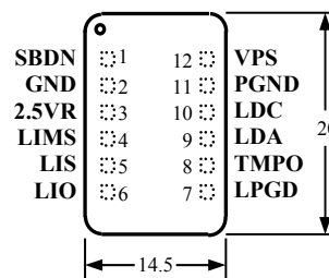
Figure 2. Pin Names and Locations
