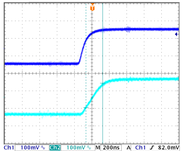
Figure 12.1. Small Signal Rise Time 192ns
