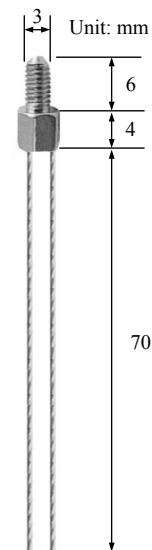
Figure 2. The Front and Side Views of ATH10KHN4
