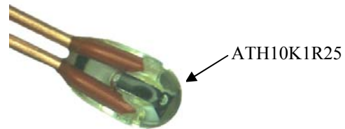
Figure 6.1. Bare Leaded Thermistor Head Photo
