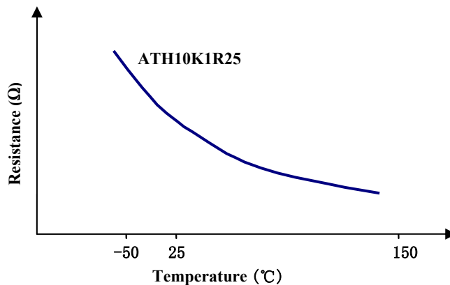
Figure 7. Resistance vs. Temperature for ATH10K1R25
