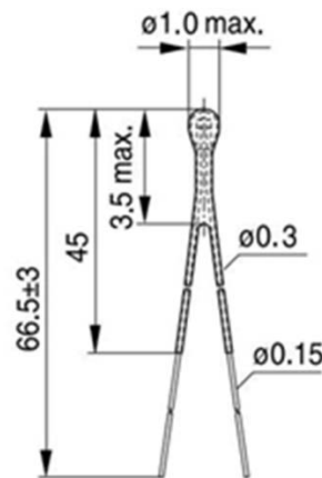
Figure 2. Side View of ATH10K1R0
