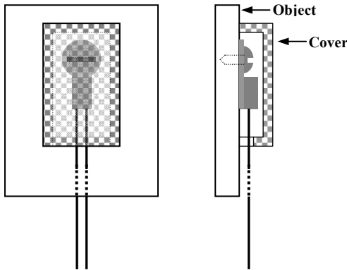
Figure 3. Using an Insulation Cover to Improve Accuracy
