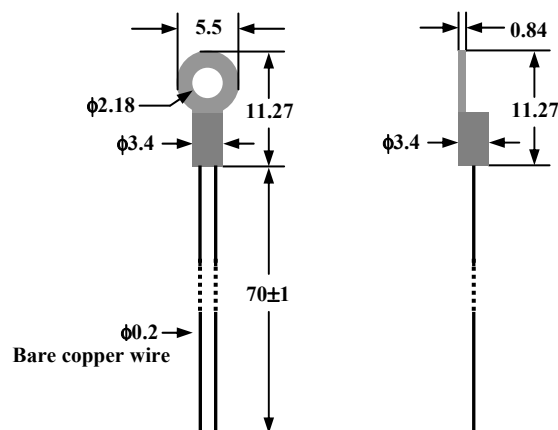
Figure 2. The Front and Side Views of ATH100KL2B
