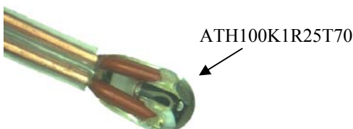
Figure 4.2. Tubing Ledged Non-sealed Thermistor Head Photo
