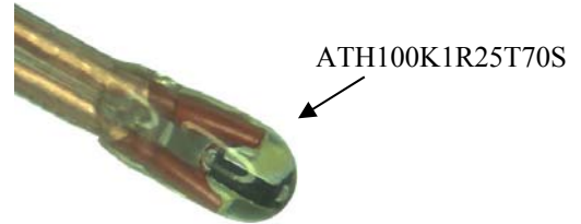
Figure 4.3. Tubing Ledded Sealed Thermistor Head Photo
