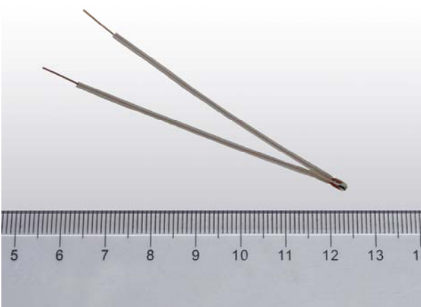
Figure 1.2 Physical Photo of the ATH100K1R25T70
