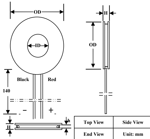
Figure 2. Mechanical Dimensions of Sealed ATE1C-49
