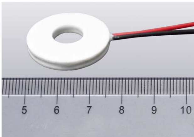
Figure 1.2. The Photo of Actual Sealed ATE1C-49
