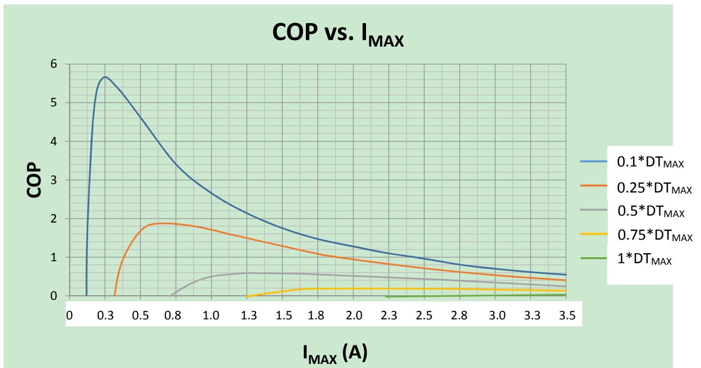
Figure 5. COP vs. I MAX
