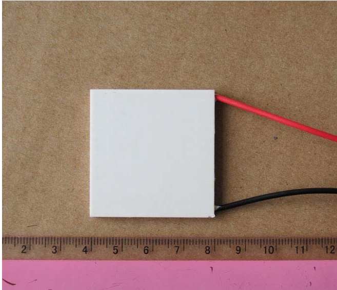
Figure 1. The Photo of Actual Sealed ATE1-97
