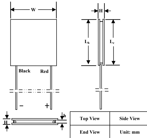
Figure 2. Mechanical Dimensions of ATE1-97
