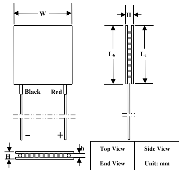
Figure 7. Mechanical Dimensions of Non-sealed ATE1-49
