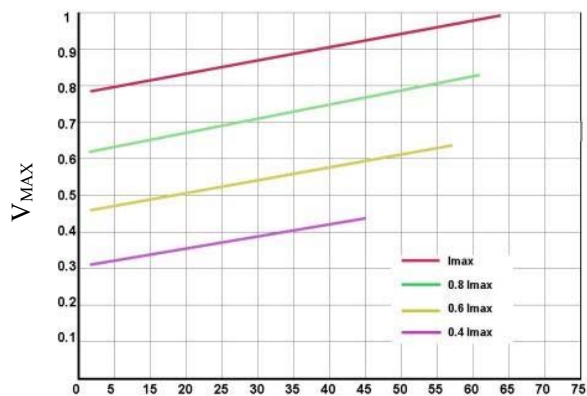
Figure 4. V_{MAX} vs. Temperature Difference
