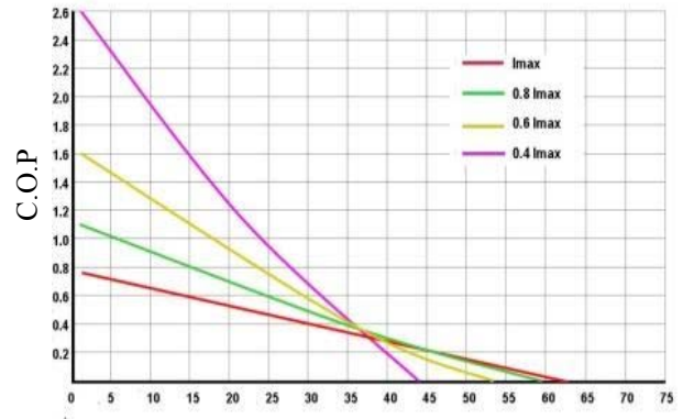
Figure 5. C.O.P vs. Temperature Difference
