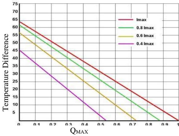
Figure 2. Temperature Difference vs. Q_{MAX}
