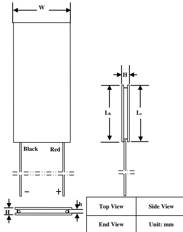
Figure 6. Mechanical Dimensions of ATE1-35
