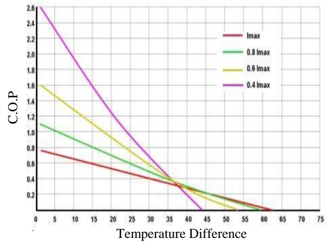
Figure 5. C.O.P vs. Temperature Difference
