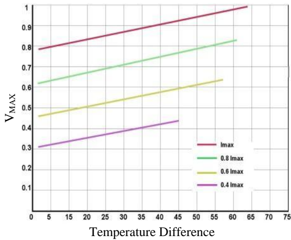
Figure 4. V_{MAX} vs. Temperature Difference
