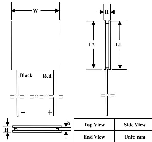
Figure 2. Mechanical Dimensions of ATE1-288
