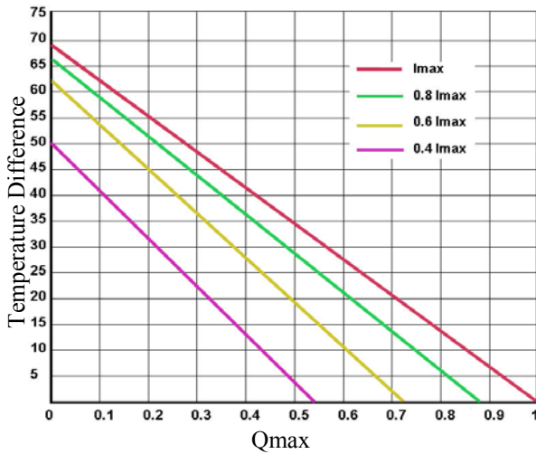
Figure 2. Temperature Difference vs. Qmax
