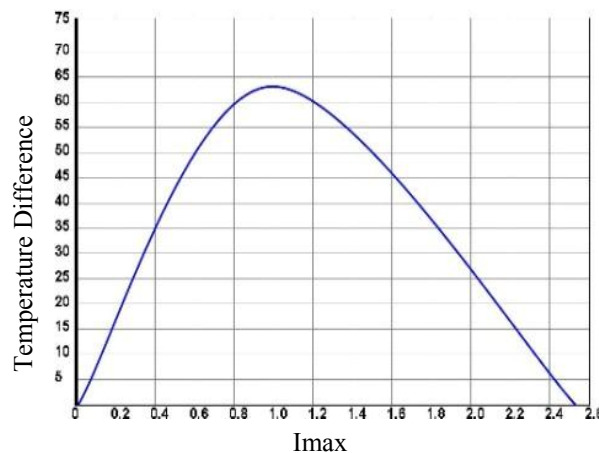
Figure 3. Temperature Difference vs. Imax
