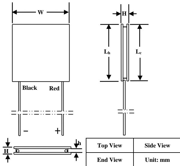
Figure 14. Mechanical Dimensions of Sealed ATE1-17
