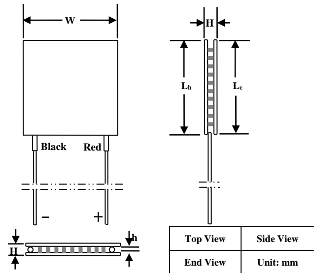
Figure 15. Mechanical Dimensions of Non-sealed ATE1-17
