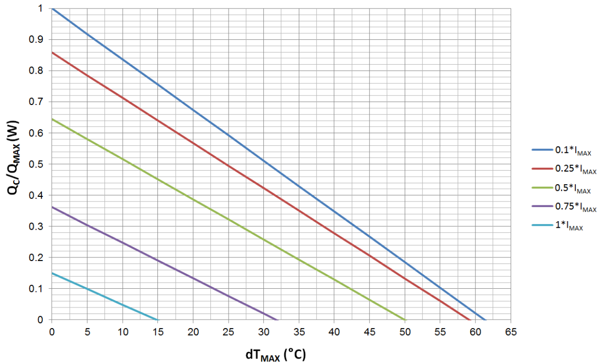
Figure 10. Q_c/Q_{MAX} vs. dT_{MAX}
