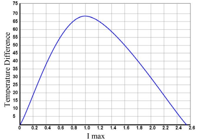
Figure 3. Temperature Difference vs. I_{max}
