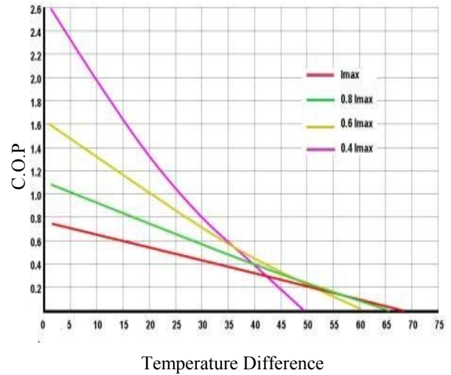
Figure 5. C.O.P vs. Temperature Difference
