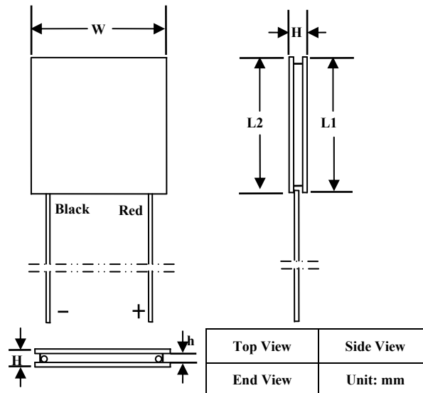
Figure 6. Mechanical Dimensions of Sealed ATE1-161 series
