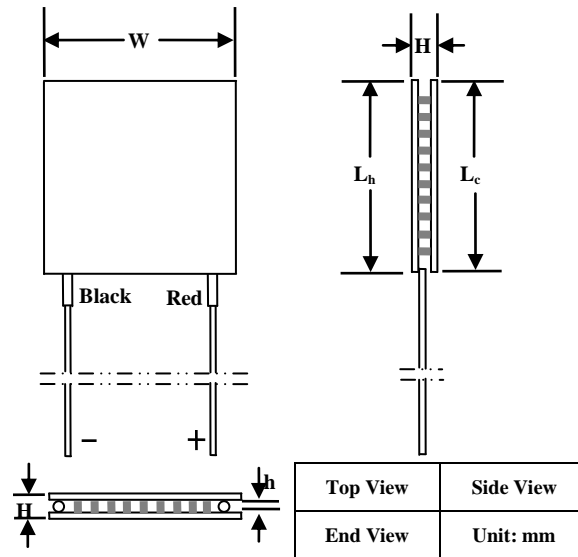
Figure 6. Mechanical Dimensions of ATE1-15-R6A
