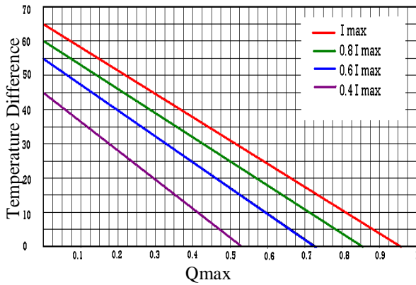
Figure 2. Temperature Difference vs. Q max
