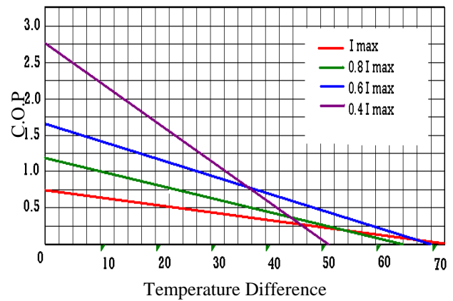
Figure 5. C.O.P vs. Temperature Difference
