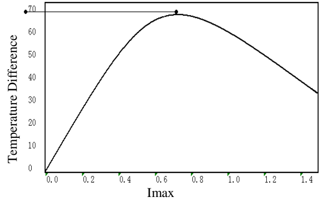
Figure 3. Temperature Difference vs. I max
