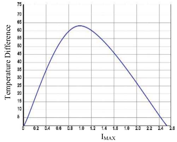
Figure 3. Temperature Difference vs. I_{MAX}
