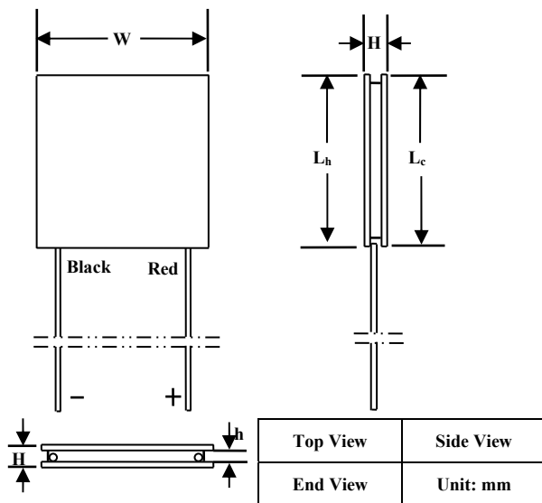
Figure 10. Mechanical Dimensions of Sealed ATE1-127
