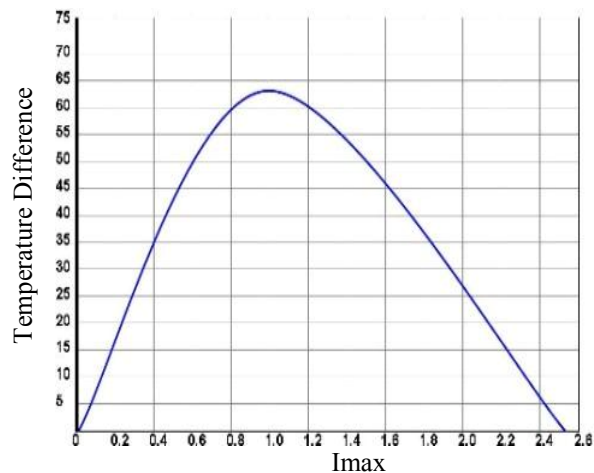
Figure 3. Temperature Difference vs. I_{max}
