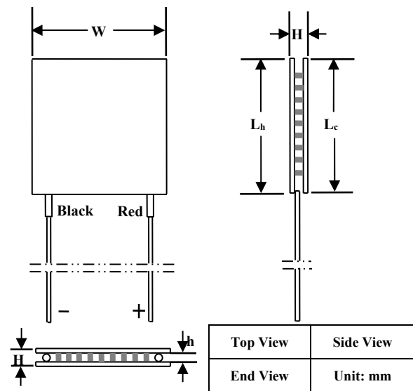
Figure 11. Mechanical Dimensions of Non-sealed ATE1-127
