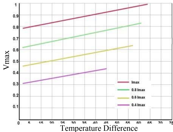
Figure 4. V_{max} vs. Temperature Difference
