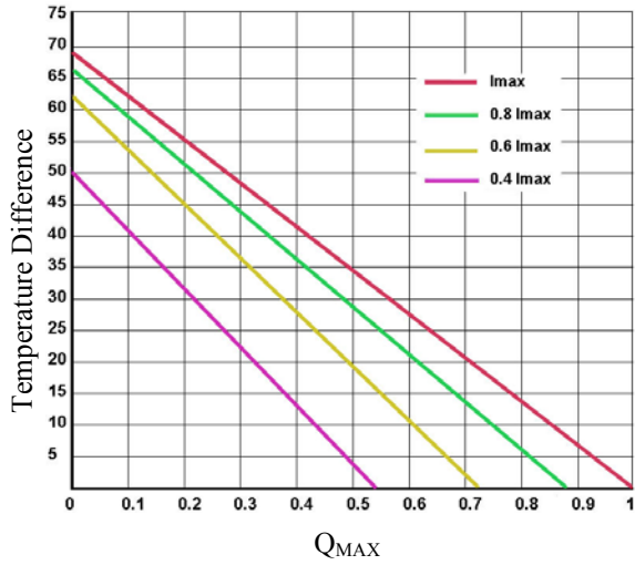
Figure 6. Temperature Difference vs. Q_{MAX}
