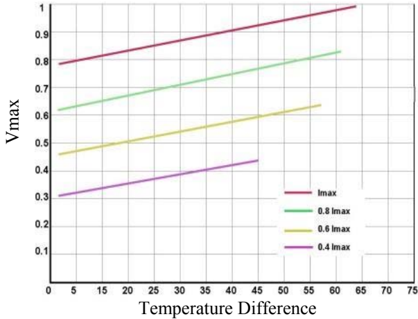
Figure 4. Vmax vs. Temperature Difference
