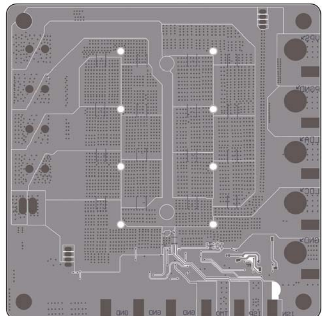
Figure 9. Mirrored Bottom Layers
