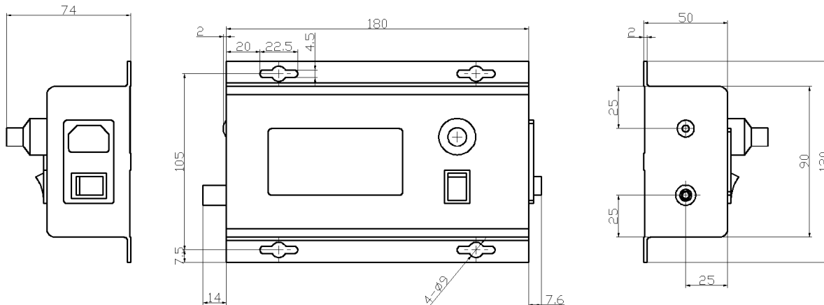
Figure 10. Dimensions for AHVACN5KV100UABT
