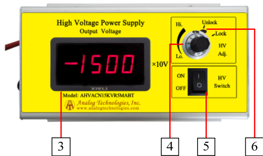
Figure 3. Front Panel
