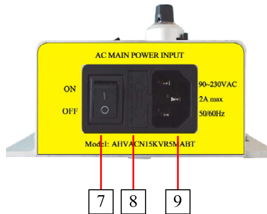
Figure 5. Right Panel
