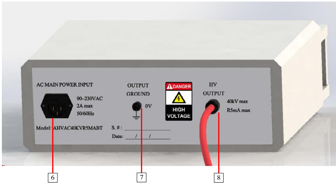
Figure 3. Front Panel
