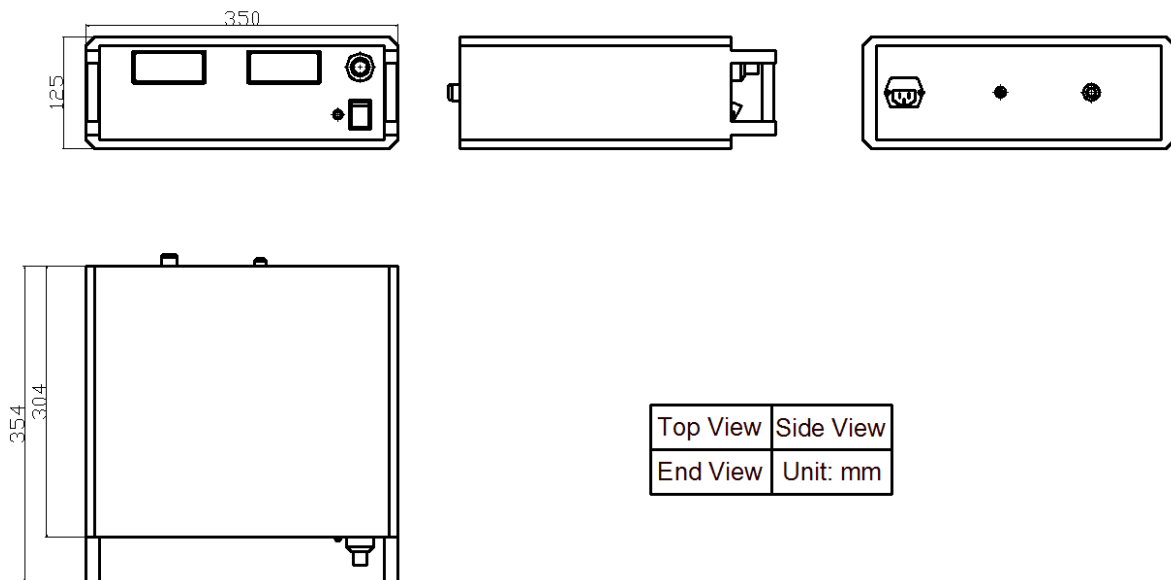
Figure 8. Dimensions for AHVAC40KVR5MABT
