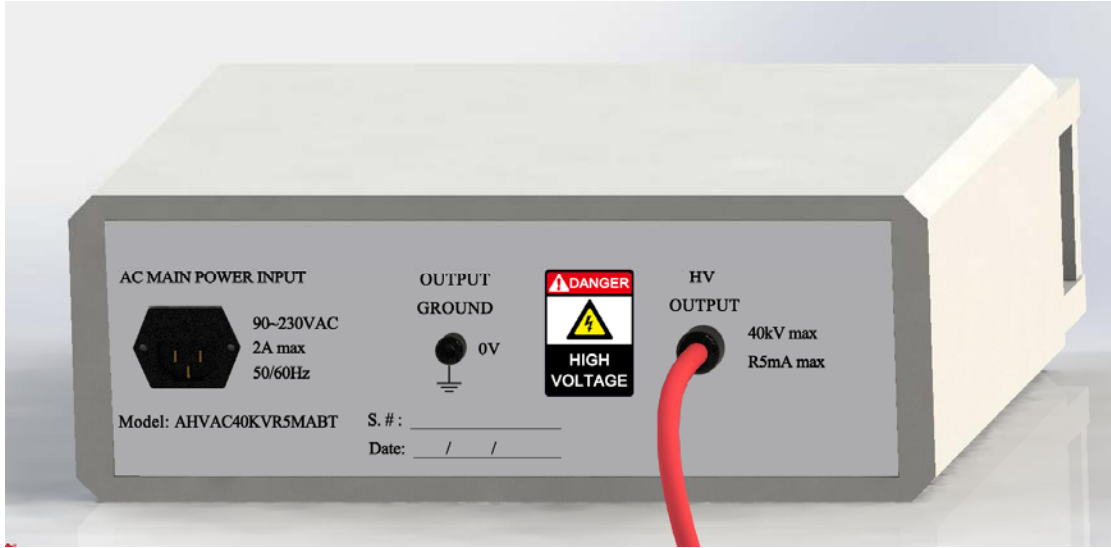
Figure 7. Leads of AHVAC40KVR5MABT
