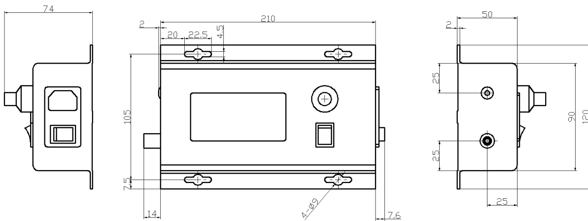
Figure 9. Dimensions for AHVAC25KVR5MABT
