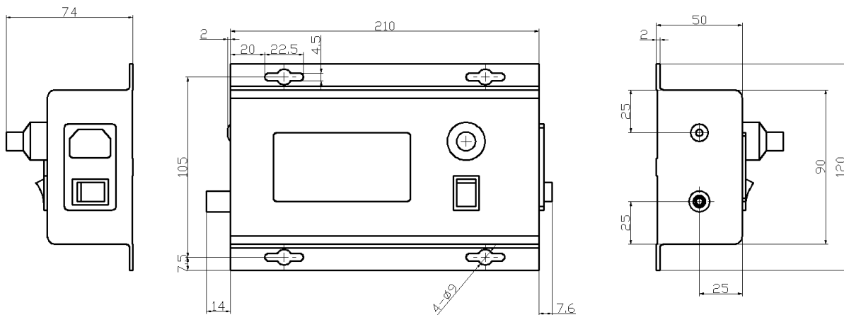
Figure 9. Dimensions for AHVAC20KVR5MABT
