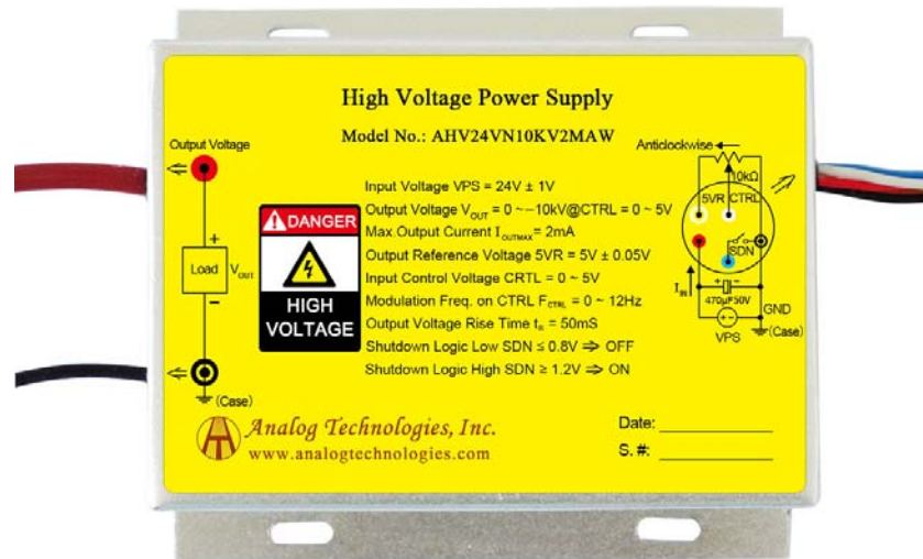
Figure 1. Physical Photo of AHV24VN10KV2MAW
