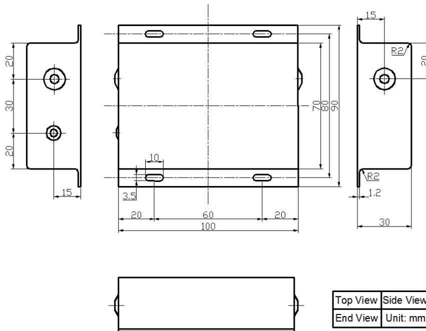
Figure 12. Dimensions for AHV24VN10KV2MAW
