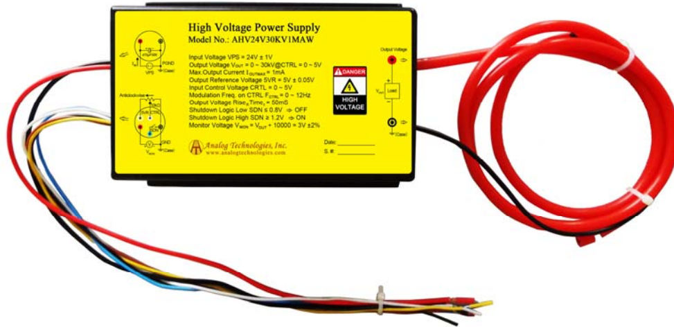
Figure 10. Leads of AHV24V30KV1MAW
