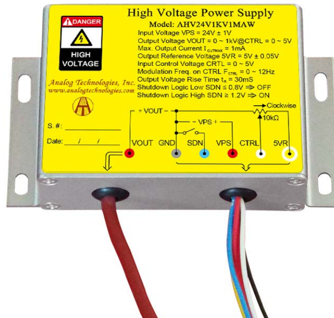
Figure 1. Physical Photo of AHV24V1KV1MAW
