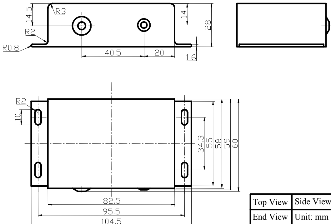
Figure 12. Dimensions for AHV24V1KV1MAW
