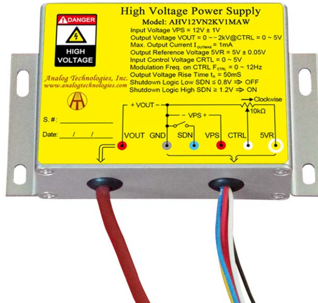
Figure 1. Physical Photo of AHV12VN2KV1MAW
