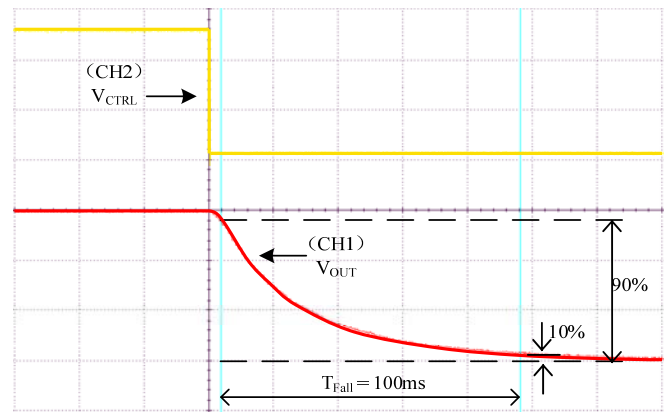
V_CTRL: 0.25V ~ 5V V_OUT: 40V ~ 1000V
