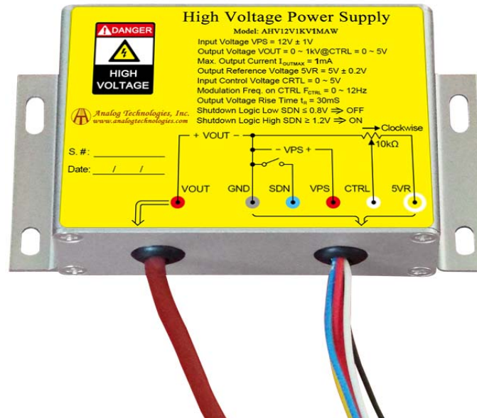
Figure 1. Physical Photo of AHV12V1KV1MAW
