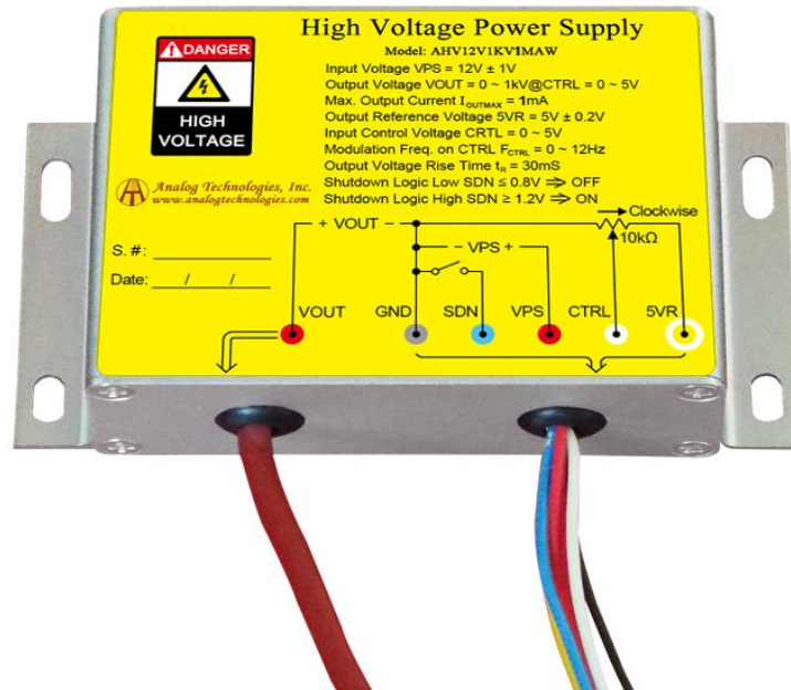
Figure 1. Physical Photo of AHV12V1KV1MAW
