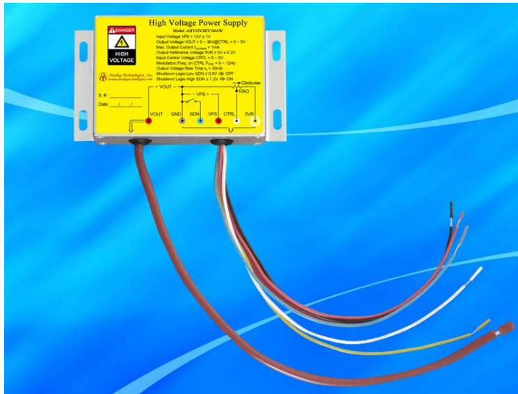
Figure 11. Leads of AHV12V1KV1MAW
