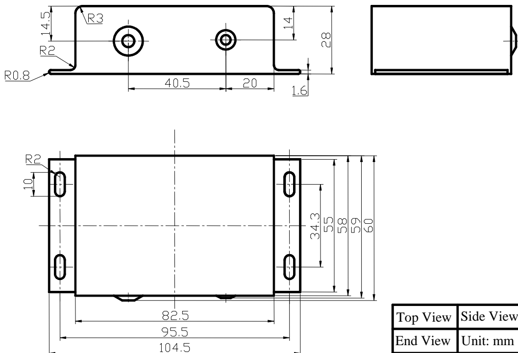
Figure 12. Dimensions for AHV12V1KV1MAW
