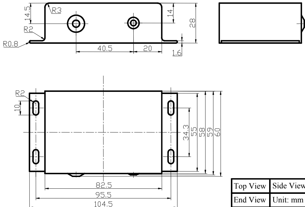
Figure 12. Dimensions for AHV12V1KV1MAW
