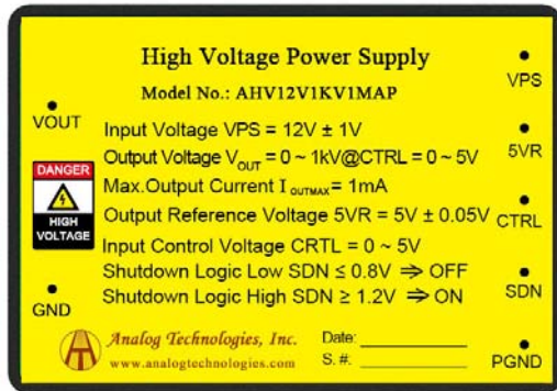
Figure 1. Physical Photo of AHV12V1KV1MAP
