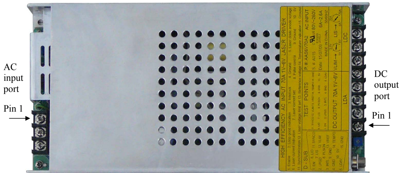
Figure 2. Top View of the AAS6V70A2
