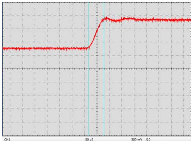
Figure 5. Digital Modulation Response at LDA Pin
