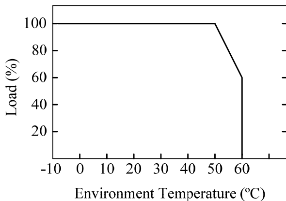
Figure 24. Derating Curve
