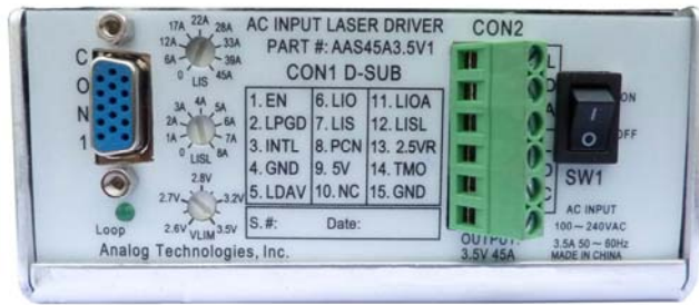
Figure 1. Front View of the AAS45A3.5V1
