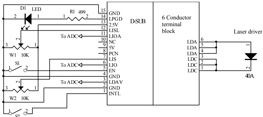
Figure 1. A Typical Application Schematic
