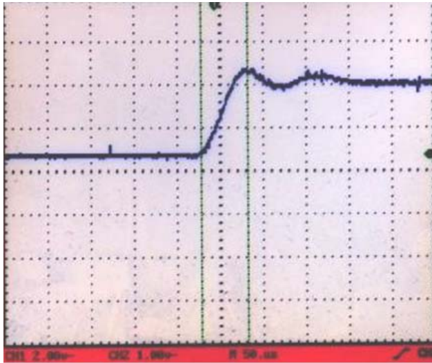
Figure 2. Digital Modulation Response at LDA Pin
