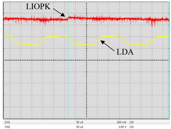
Figure 20. Digital Modulation Response at LIOPK & LDA Pin (f=4kHz)
