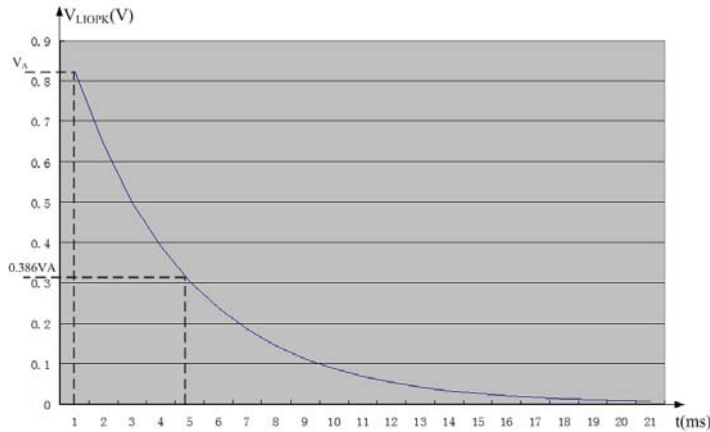
Figure 6. LIOPK's Mathematic Model
