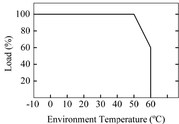
Figure 26. Derating Curve
