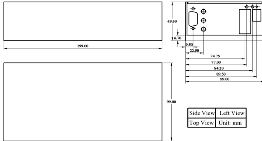
Figure 29. Mechanical Dimensions
