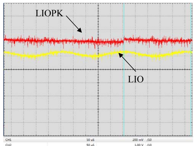
Figure 21. Digital Modulation Response at LIOPK & LIO Pin (f=4kHz)
