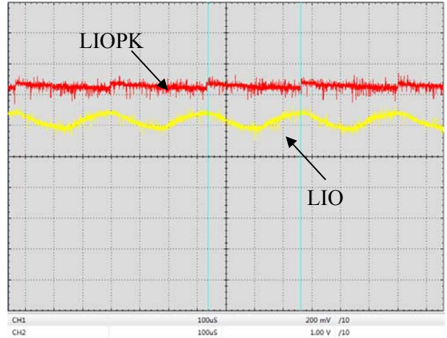
Figure 19. Digital Modulation Response at LIOPK & LIO Pin (f=3kHz)
